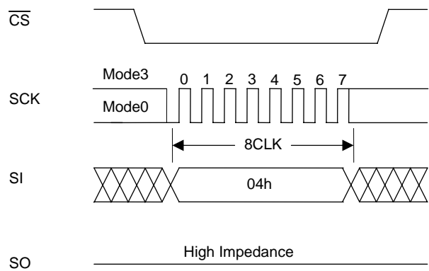
Figure 12 Write Disable
